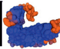
3D structure of CMPG1 of Solanum lycopersicum
