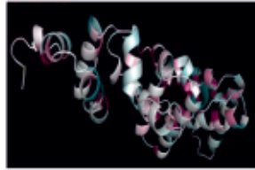
3D structure of RxLR 29
