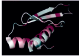
3D structure of DRB4 from Arabidopsis thaliana
